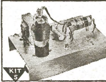
KIT 5 Building this A. M. Signal Generator gives you more valuable experiences. It provides amplitude-modulated signals for many tests and experiments.
